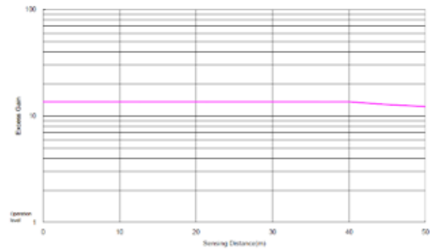
EXCESS GAIN - THROUGH BEAM
