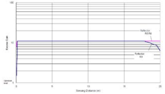
EXCESS GAIN - POLARISED RETROREFLEX
