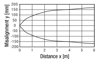
Typ. response behavior (TK 100x100)
