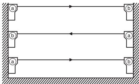
Figure 6.1: Multi-axis arrangement
