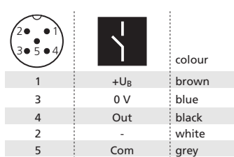
Fig. 1: Pin assignment with view onto sensor plug and colour coding of the Balluff connection cables
