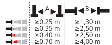
Fig. 2: Assembly distances
