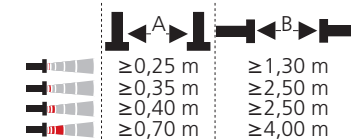
Fig. 2: Assembly distances
